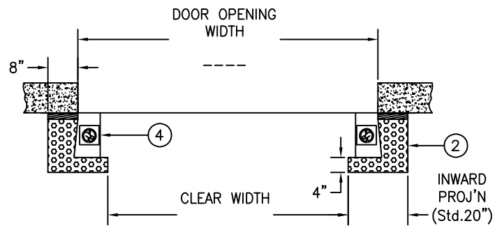
CROSS SECTION
